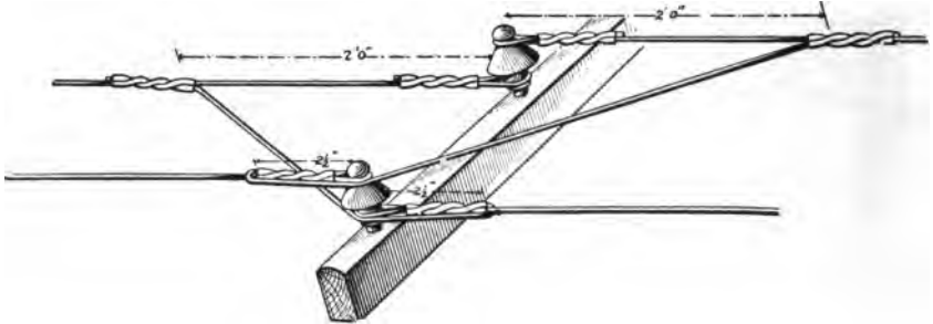
FIG. 126.—Line transposition.
